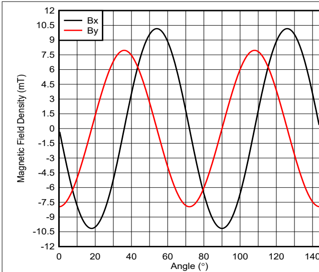
Figure 3-3. Magnetic Field Components
