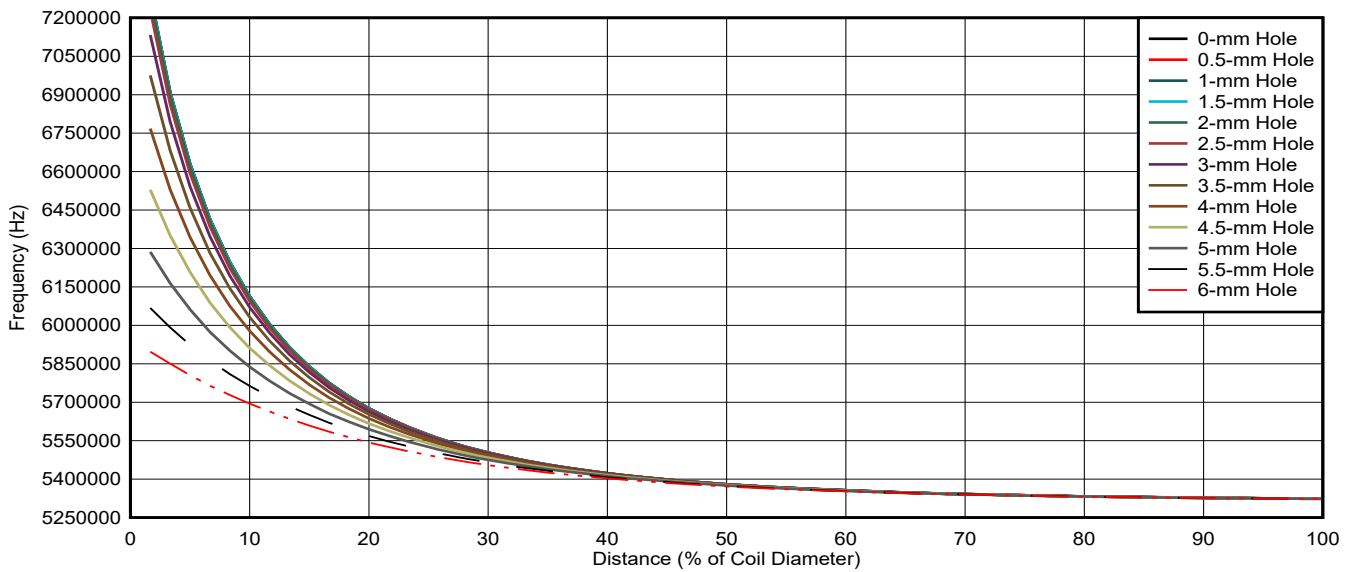
Figure 2-11. Hole Size Comparison
