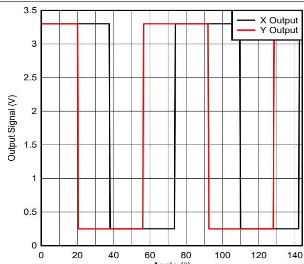
Figure 3-4. TMAG5110 Output
