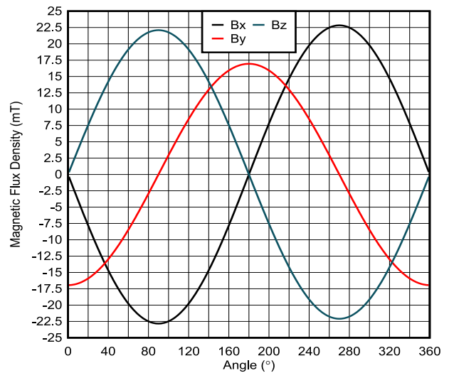
Figure 3-10. Scroll Wheel Sensor Magnetic Fields: Out-of-Plane Sensor
