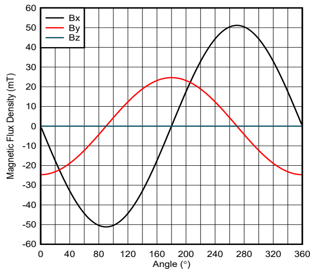
Figure 3-9. Scroll Wheel Sensor Magnetic Fields: In-Plane Sensor
