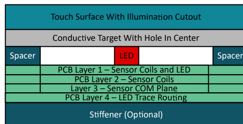
Figure 2-12. Inductive Touch Button With Center LED Stackup
